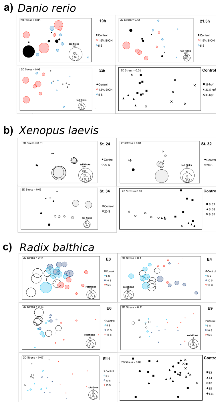
Figure 3 Multidimensional scaling plots in two dimensions using Bray-Curtis similarity matrices. MDS plots using Bray-Curtis similarity matrices performed on logarithmically transformed spectral frequency data produced using Discrete Fourier Transform analysis of (i) negative angle (ii) positive angle (iii) centre of mass – rho and (iv) centre of mass – theta, frame-to-frame parameters for (a) Danio rerio , (b) Xenopus laevis and (c) Radix balthica under different environmental conditions and at different developmental stages. Bubble size represents the amount of tail flicks of Danio rerio and Xenopus laevis , the number of rotations of Radix balthica at stages E3, E4 and E6, and the number of complete gliding along the circumference of the egg capsule on stages E9 and E11.
