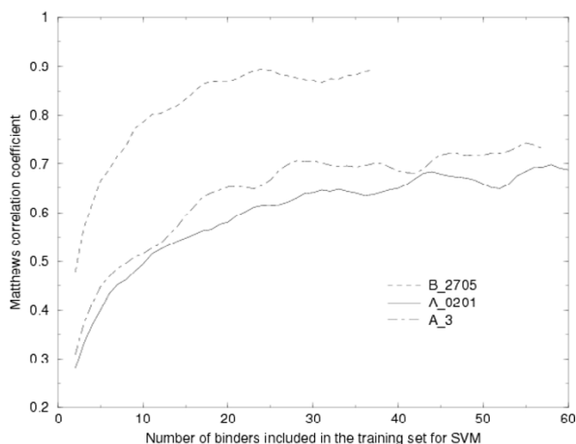
Figure 1 Performance of SVMHC for the MHC type HLA-A*0201, HLA-A3 and HLA-B*2705, measured by the Matthews correlation coefficient, Mc, versus the number of peptides used for training. For all sizes of the training-set the test-set was identical and no part of the test-set was contained in the training-set.
