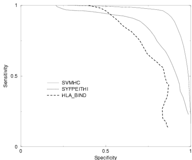
Figure 2 Specificity/sensitivity plots for SVMHC HLA_BIND and SYFPEITHI. Sensitivity is defined as the number of correctly predicted binders (TP) found at a given cutoff, divided with the total number of binders, i.e. Sens = TP / (TP + FN) , where FN is the number of . The specificity is defined as the fraction of the hits above this cutoff that is correct, i.e. Spec = TP / (TP + FP) . It can be seen that the sensitivity of SVMHC is higher than of SYFPEITHI and HLA_BIND at any specificity.
