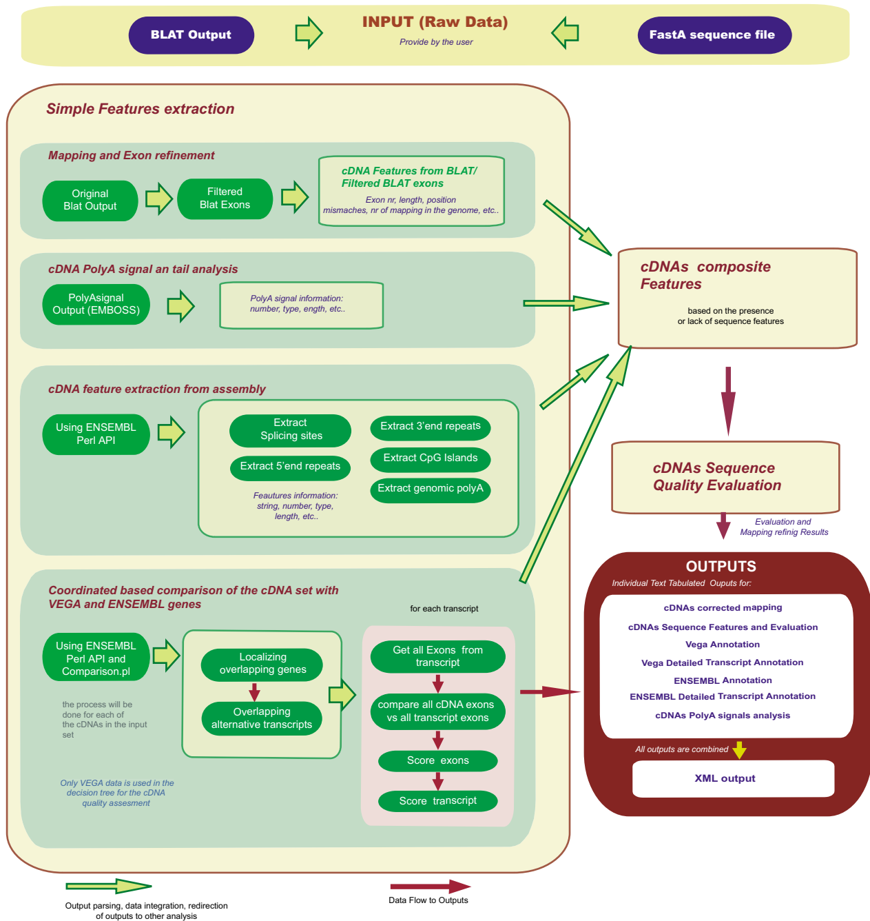
Figure 1 Caftan pipeline, data and program flow.
