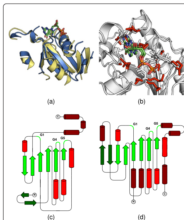
Figure 6 Alignment of the Dynamin A GTPase domain and the cpGTPase domain from the YjeQ. Topologies of (a) the Dynamin A GTPase (SCOP domain d1jwyb_) and (b) cpGTPase domain from the YjeQ protein (d1u01a2). Aligned SSEs are indicated by lighter colors. (c) DEDAL superposition of the GTPase and the cpGTPase domains (yellow and blue, respectively). For clarity, only the aligned parts of the structures in the same superposition showing residues participating in the GDP/GTP binding (red) and the GDP molecule. Despite significant topological differences, DEDAL effectively handles all alignable SSEs and correctly superimposes the active sites. The sequence identity of the superimposed regions is 24.2%.
