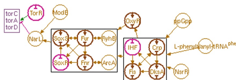
Figure 5 The Genetic Regulation Schematic for the E. coli torCAD operon.
