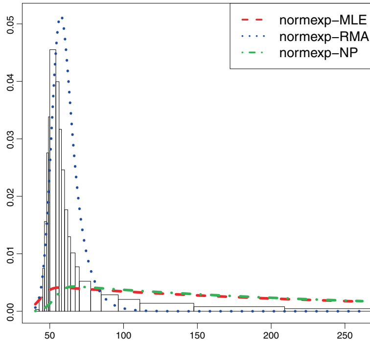
Figure 1 Normal-exponential fit. Normal-Exponential estimation for one array from (E_1) after removal of imperfectly designed probes: irregular density histogram of all regular probe intensities and the plug-in normexp density of the regular probes with MLE, RMA and NP parameter estimates.
