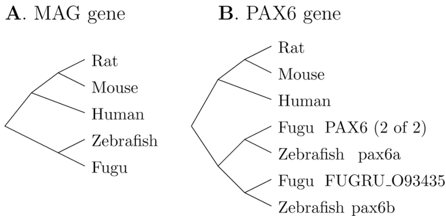
Figure 3 Gene trees. Gene trees for the MAG and the PAX6 gene families across five species.
