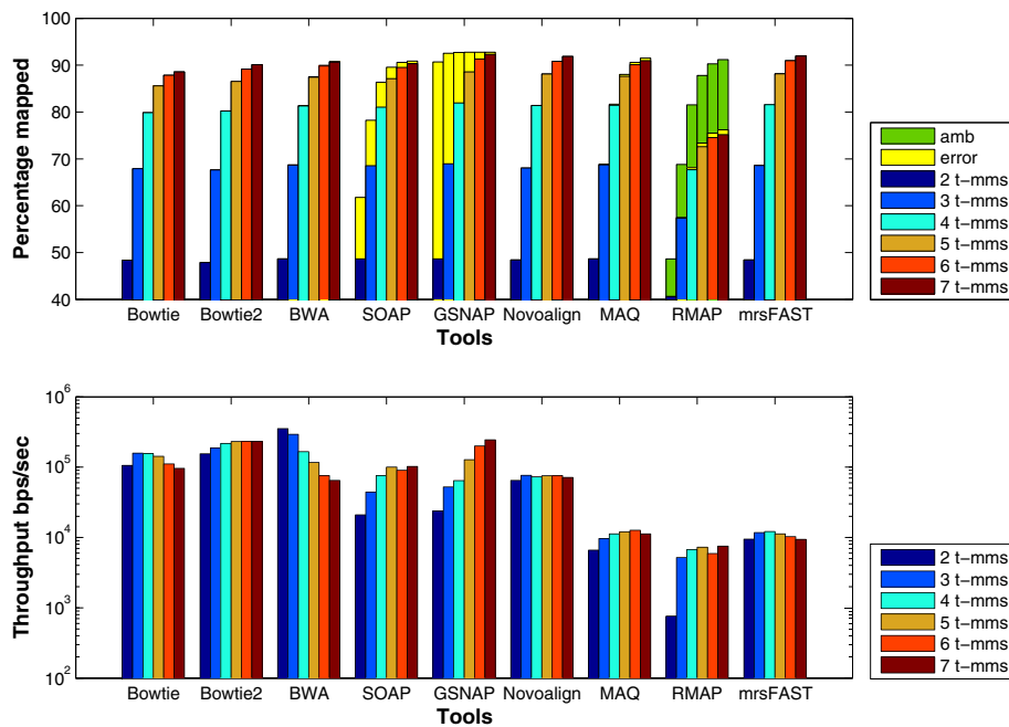
Figure 5 Effect of changing the number of mismatches using a synthetic data set extracted using wgism . Comparing the different tools while changing the total mismatches from 2 to 7. T-mms stands for the maximum allowed mismatches. A data set of 1 million reads of length 125 extracted from the Human genome using wgism was used in this experiment.
