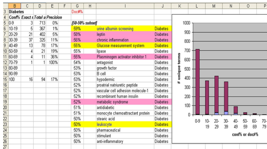
Figure 4 PubMed results confidence levels x I2E-manual precision. Correlation between InfoCodex confidence levels (Conf%; purple bars) and precision (light blue bars) against I2E-manual diabetes PubMed benchmark. Pink shading: exact match; yellow shading: partial match. Row 15 (100 Conf%) represents a member of the manually compiled reference set.
