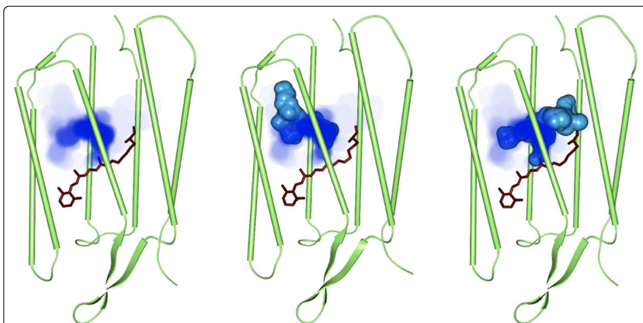
Figure 9 Residence probability of a single dynamic cavity in bacteriorhodopsin. The residence probability of the traced dynamic cavity is displayed using the maximum intensity projection. In the middle and right images, the static cavities together with the dynamic cavity at two different time steps are shown as skin surface.
