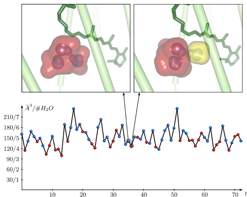
Figure 7 Single cavity tracing. Bottom: Volume plot of a single cavity traced over 72 time steps. The point color highlights whether two (red) or three (blue) water molecules are contained in the cavity. The labeling of the y-axis gives the volume numbers as well as the corresponding water molecules that would approximately fit into the volume, where the volume of a water molecule is approximated by 30 \text{ \AA}^3 . Top: The two images on top of the graph show the traced cavity (red) for two selected time steps together with the contained water molecules. In the right image, it can be seen that the traced cavity has split. A second, smaller cavity (yellow) contains the third water molecule.
