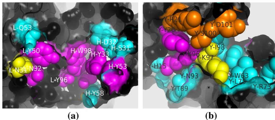
Figure 3 Prediction results by \beta ACV_{ASA} for the residues in the interface between Chain Y and Chain HL(together) in 3HFM. In (a) and (b), the true predicted hot spot residues are in magenta, the false predicted non-hot spot residues are in yellow, the false predicted hot spot residues are in orange, while the true predicted non-hot spots are in cyan; X-YZZ stands for residue Y in position ZZ of Chain X.
