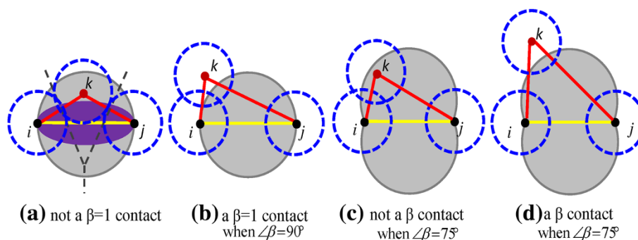
Figure 1 Examples of \beta contacts and non- \beta contacts. Three points, denoted by i, j and k , represent atoms. The dashed circles represent the van der Waals spheres in 2D space. The lines in yellow are of interest.
