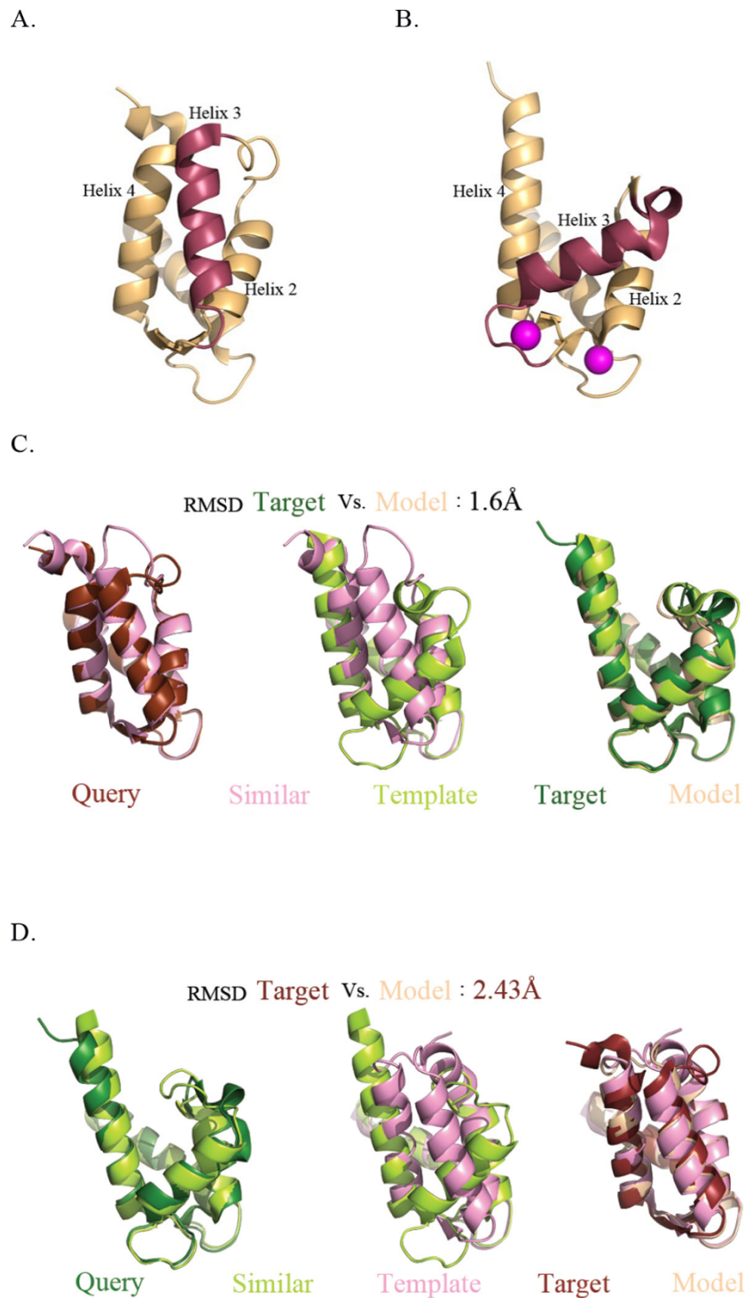
Figure 1 ConTemplate results demonstrated using the S100A6 Ca 2+ binding protein. The Ca 2+ -free (A) and -bound (B) conformations are shown in the upper panels; helix 3 is marked in red, and the calcium ions in magenta. C. Reproducing the Ca 2+ -bound conformation, starting from the Ca 2+ -free conformation as a query. The maximal RMSD between the query and similar proteins is set to 1.2Å, the minimal Q-score to 0.4, and the number of clusters is set to 2. D. Reproducing the Ca 2+ -free conformation, starting from the Ca 2+ -bound conformation as a query. The similarity cutoffs are the same as in C, the number of clusters is set to 17.
