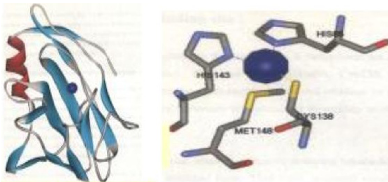
Figure 1 a) Rusticyanin bound to the copper atom as indicated by the blue colored ball. b) Copper binding active site of rusticyanin showing the four active site residues: Histidine at 85 th position, Histidine at 143 rd position, Cysteine at 138 th position and Methionine at 148 th position
