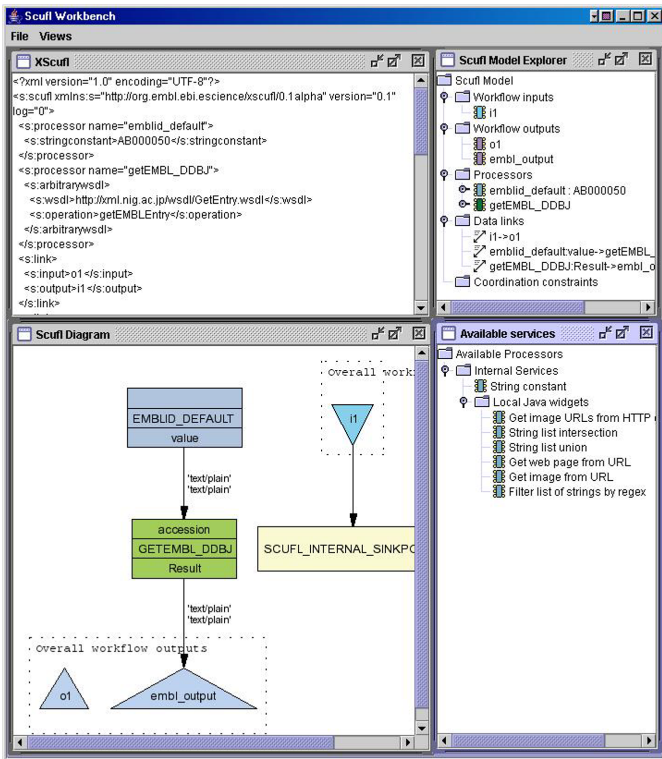
Figure 3 Taverna, the Scufi Workbench Screenshot of Taverna implementation of RPC based workflow retrieving EMBL information from DDBJ.
