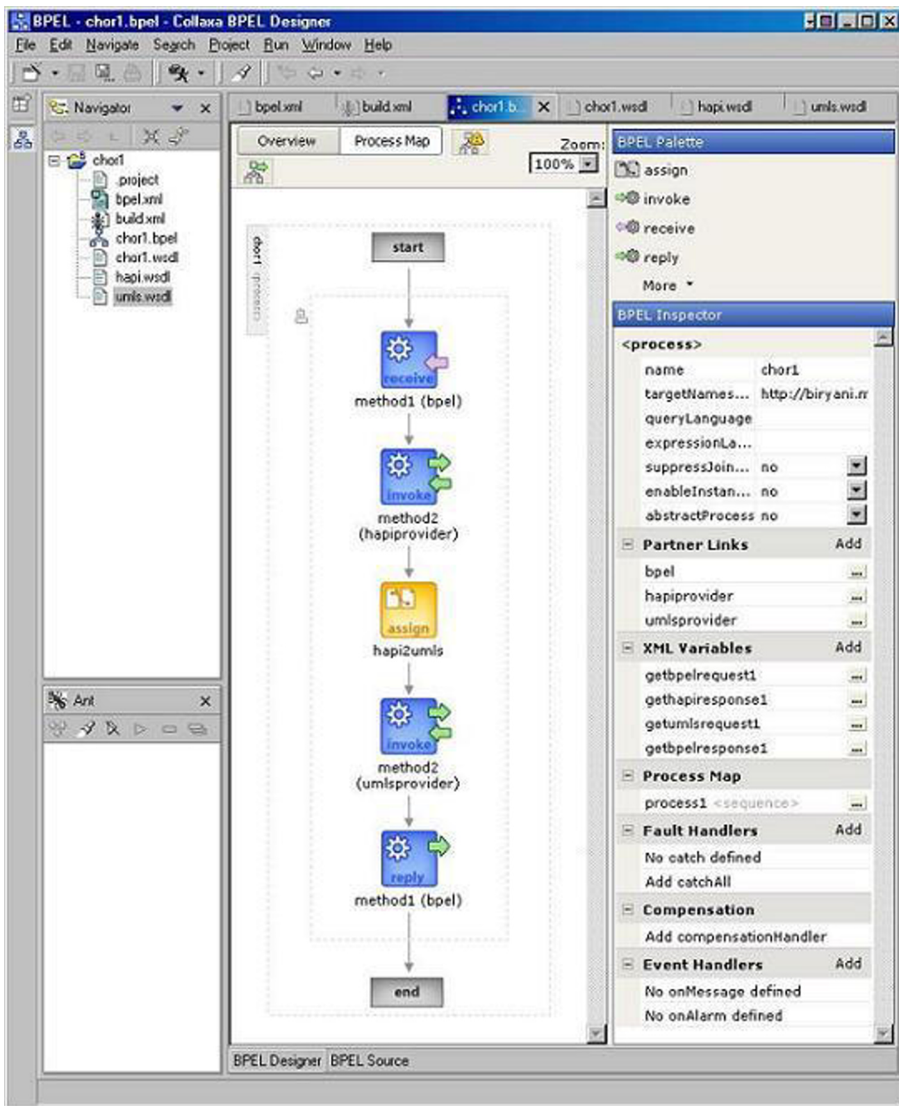
Figure 4 Collaxa BPEL Server Screenshot of Collaxa's bpelez design tool, building a choreography of GetHAPI and GetUMLS web services
