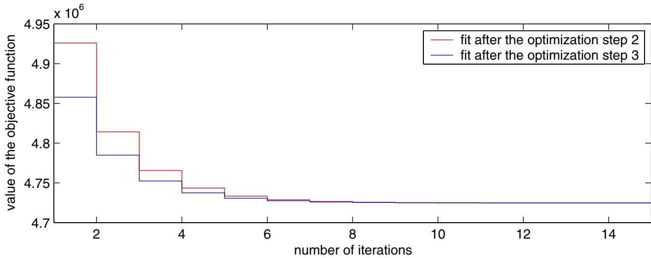
Figure 3 Evolution of the value of the objective function. The red (resp. blue) graph corresponds to the value of the objective function after step 2 (resp. step 3).
