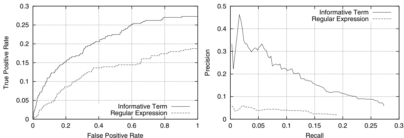
Figure 4 ROC and precision-recall graphs for predictions made by the system. ROC and precision-recall graphs for GO code predictions made by the system aggregated over the three ontologies. The solid line represents predictions made by the Informative Term/Naïve Bayes path in Figure 1. The dashed line represents predictions made by the Regular Expression/Naïve Bayes path in Figure 1.
