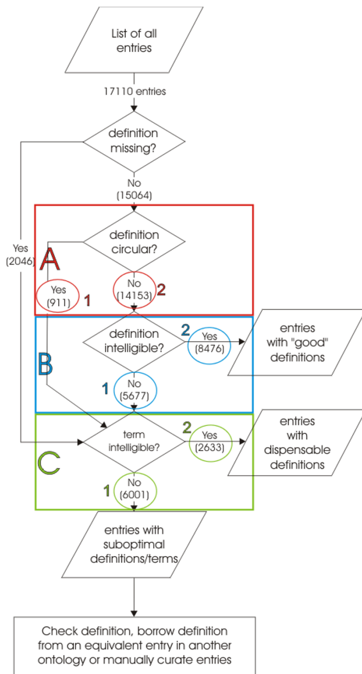
Figure 1 Workflow for the computational evaluation of the quality of terms and definitions in controlled vocabularies.
