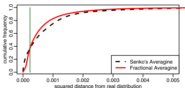
Figure 3 Comparison of the impact of averagine and fractional averagine stoichiometry estimation errors on the estimation of theoretical isotope distributions. The cumulative histograms of least squares deviations from the true theoretical isotope distribution illustrate the superior overall performance of fractional averagine (solid line) compared to Senko's classical averagine (dashed line): fractional averagine causes a 17% decrease in mean squared error magnitude.
