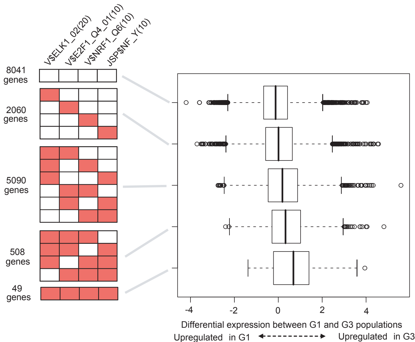
Figure 3 Dependency of differential expression between G1 and G3 breast tumors on sequence features. Genes are divided into five groups based on patterns of four sequence features, V$ELK1_02(20), V$E2F1_Q4_01(10), V$NRF1_Q6(10) and JSP$NF_Y(10) (the left red boxes indicates the presence of sequence features). The distributions of their differential expression values between G1 and G3 are displayed using box plots.
