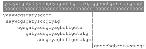
Figure 6 Output of PAMPS for a set of 20 sequences, given l_{min} = 17 and d_{max} = 64 (gray background). In this case the output is a single sequence which is split just before a G nucleotide that is marked by | underneath it. Each nucleotide belongs to at least a sub-sequence of length at least 17 and degeneracy at most 64 which does not pass over the split point (the split point is indicated by the vertical dashed line; see Methods for description of split point). All sub-sequences that meet these criteria are indicated below the output. Obviously not all sub-sequences of length 17 nt have degeneracy less than 64. The possibility of choosing between several sub-sequences allows the user to design more compatible pairs of primers, e.g. primers with close annealing temperatures.
