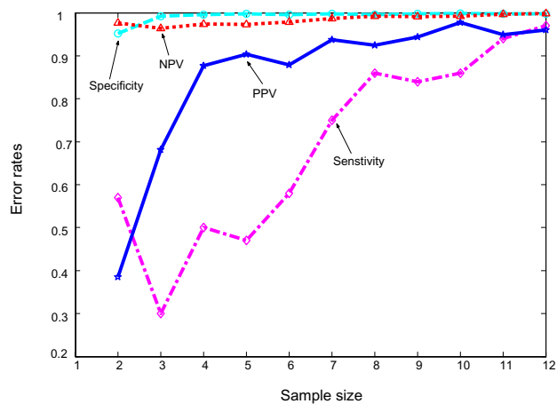
Figure 3 Effect of sample size on error rates in the multiple testing in our simulation study. Effect of the sample size on error in multiple testing with the GLRT to identify the DE genes under the multivariate hierarchical model. The x-axis is the number of replications and the y-axis is the error rates. The sensitivity is expressed by diamond, specificity by circle, PPV by star and NPV by triangle.
