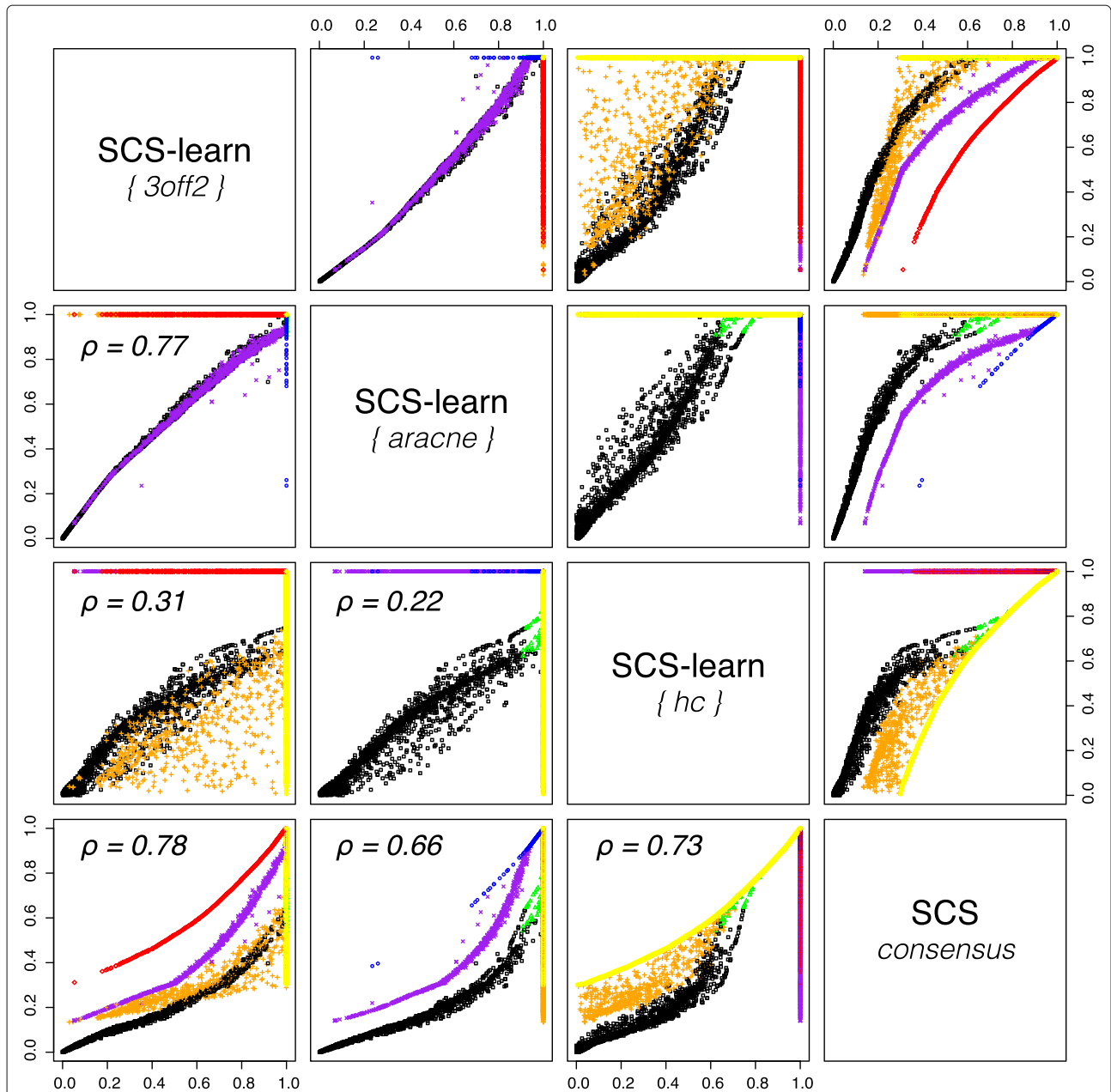
Fig. 4 Edge rank correlations between SCS-learn and SCS-consensus outcomes for human gut microbial ecosystem. 6,389 edges were predicted from a dataset of 663 observations and 2,101 CAGs (MetaHIT project [47]). Rank of edges predicted by only one embedded learning method are given in blue (ARACNE, 159 edges), red (3off2, 498 edges) and yellow (hill-climbing, 2,889 edges). Rank of edges predicted by two individual learning methods are given in green (ARACNE & hill-climbing, 31), orange (3off2 & hill-climbing, 573 edges) and purple (3off2 & ARACNE, 720 edges). Rank of edges predicted by all individual methods are given in black (1,519 edges)
