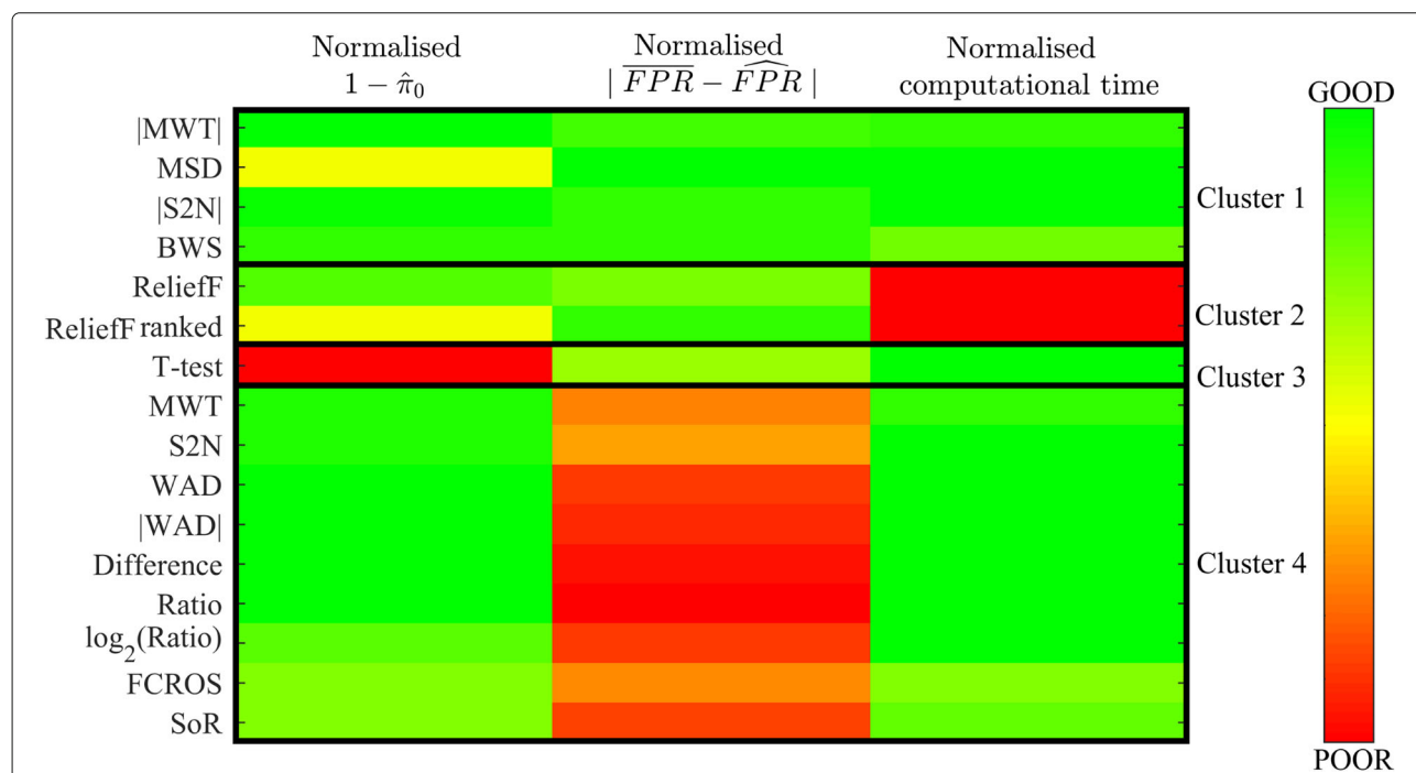
Fig. 2 Results of k-means cluster analysis based on three performance criteria. Results highlighted with green colour show good performance, red colour represents poor performance and yellow colour represents medium performance
