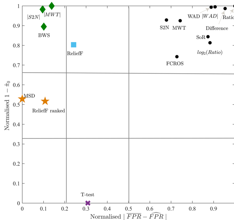
Fig. 3 Results of k-means cluster analysis based on two performance criteria. The best results have those metrics, where FPR estimation is closest to 0, and sensitivity estimation ( 1 - \widehat{\pi}_0 ) is closest to 1
