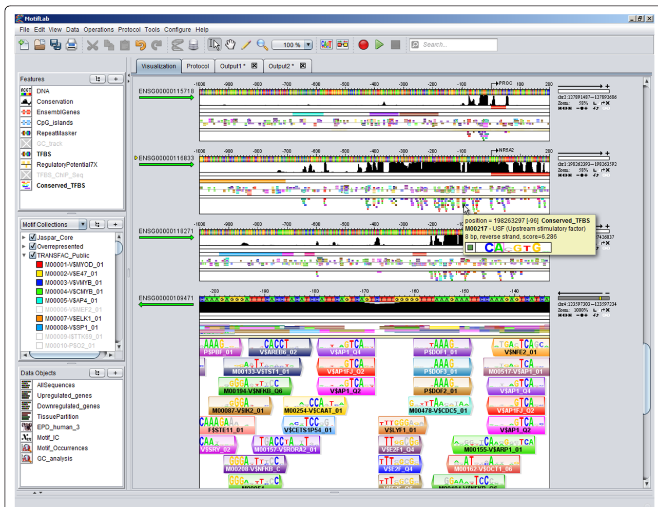
Figure 1 MotifLab's graphical user interface. The screenshot shows MotifLab's graphical user interface with three data panels to the left and with the sequence browser to the right taking up most of the screen space. The top data panel contains the feature datasets in the order they are visualized as tracks in the sequence browser, the middle data panel contains the motifs and modules, and the bottom panel contains miscellaneous data objects that do not belong in the first two panels. Features and motifs that are greyed out in the data panels are hidden from view in the sequence browser. The bottommost sequence shows a motif track in "close-up mode" which is activated at zoom-levels above 1000%. The binding sites are shown with superimposed "match logos" where the base matching the DNA sequence in that position is shown in colour and the other three bases are greyed out.
